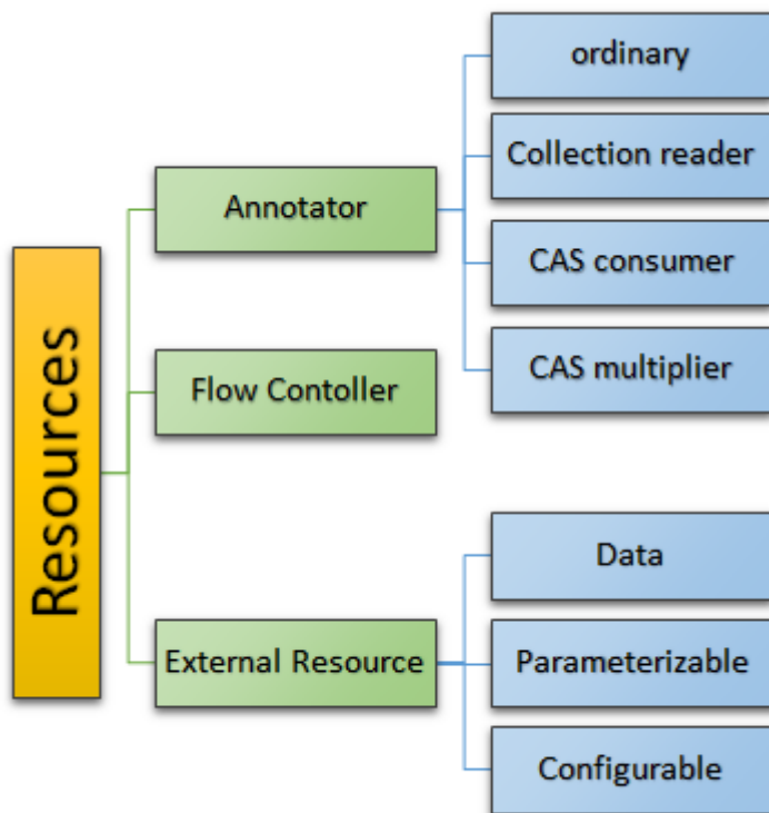
Figure 5. Resource Kinds
